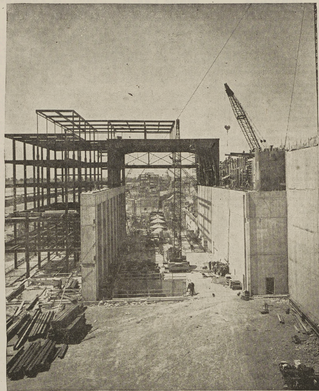
HYDRO BUILDING WELL ADVANCED — In this unusual picture, the powerhouse construction in the background is framed by the structural steel of the administration building which is situated on the north end of the power dam. All the structural steel for the powerhouse erection bay and administration building now is virtually erected. —Ontario Hydro Photo
